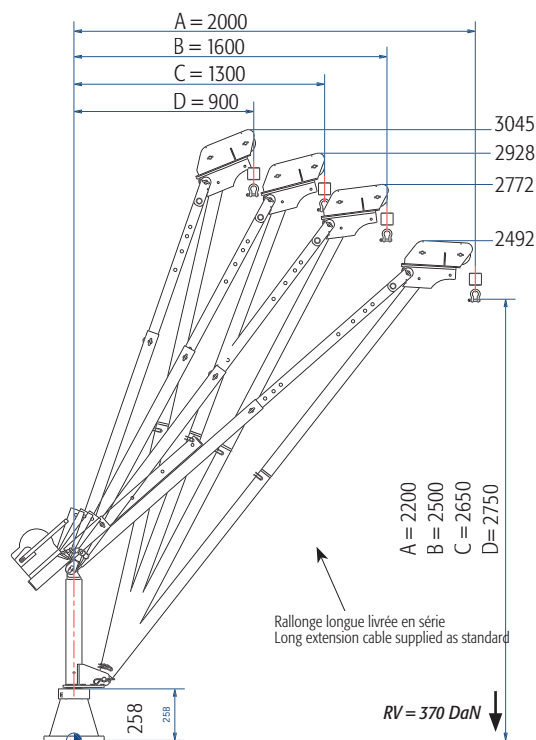
1 POTENCE = 2 MODES D'ASSEMBLAGE POSSIBLES | 1 JIB CRANE = 2 POSSIBILITIES
