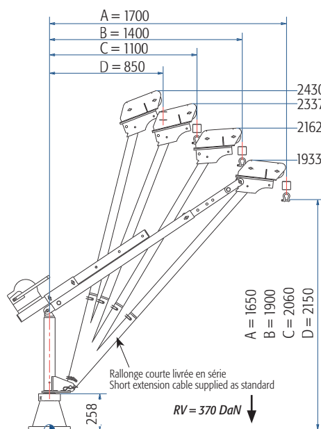
1 POTENCE = 2 MODES D'ASSEMBLAGE POSSIBLES | 1 JIB CRANE = 2 POSSIBILITIES
